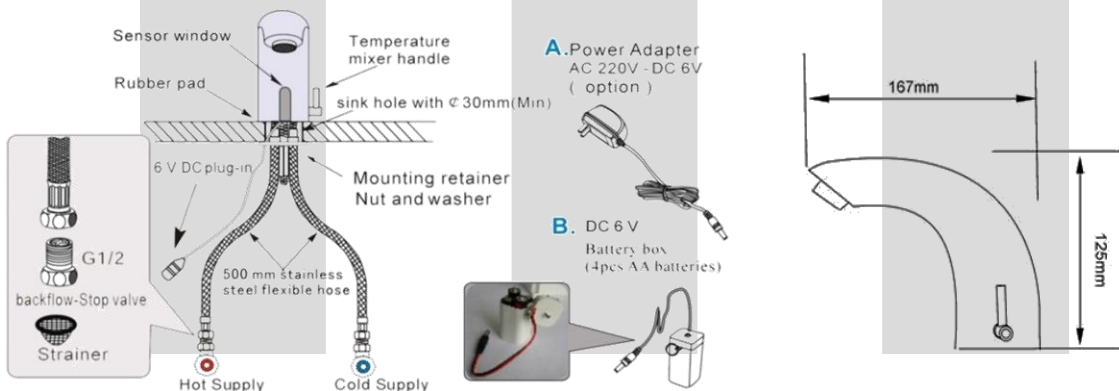
CAT 67913 MIXER AUTO FAUCET
