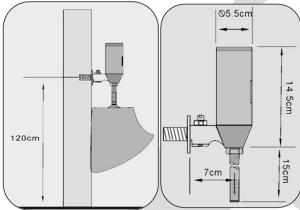
CAT 67 106 AUTO URINAL VALVE
