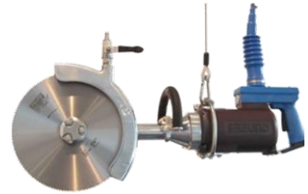
CAT 202 SK28 280 mm 14 KG
