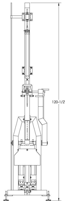
CAT 143 31 HEAD CHISELOR AND JAW PULLER – ON RAIL
