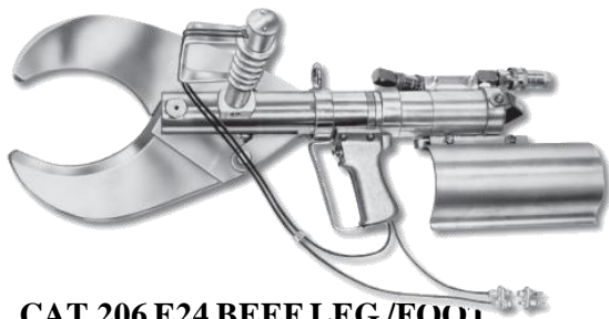
CAT 206 E24 BEEF LEG / FOOT SHEAR
