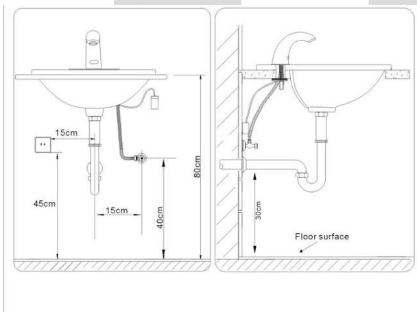
CAT 67801 AUTO WASHROOM SPOUT
