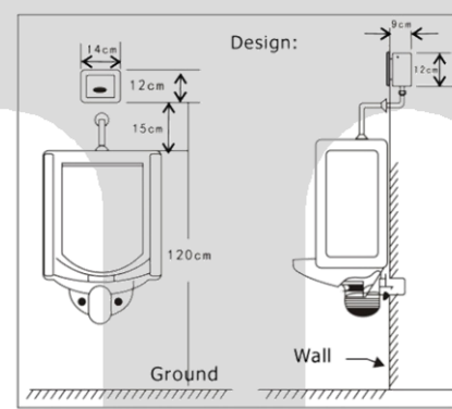
CAT 67201 AUTO/URINAL TOILET FLUSH
